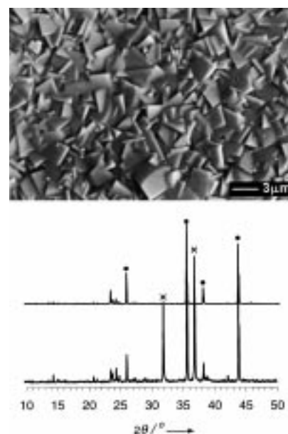
Figure 6. Top) SEM image of a ZSM-5 film prepared conventionally on a seeded alumina substrate placed in a 10 mL reactor. The reaction was carried out for 16 h at 180^\circ\text{C} in a clear solution of composition \text{SiO}_2:0.5\text{NaOH}:1/300\text{Al}_2\text{O}_3:80\text{H}_2\text{O} . Bottom) X-ray diffraction pattern of the film (top curve), compared with that of a film prepared by parallel synthesis (bottom curve). The peaks marked with a dot originate from the alumina substrate, and the peaks marked with a cross from the lead mask.
